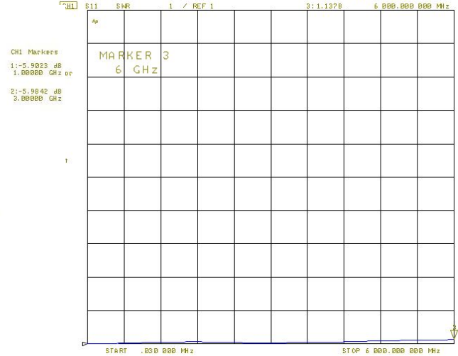
6dB Attenuator, S21 / VSWR
