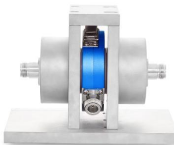
Picture 2: TBCP2-CAL RF current probe calibration fixture
