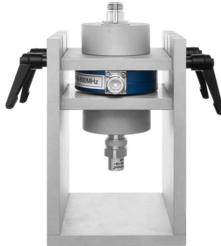
Picture 2: TBCP4-CAL RF current probe calibration fixture
