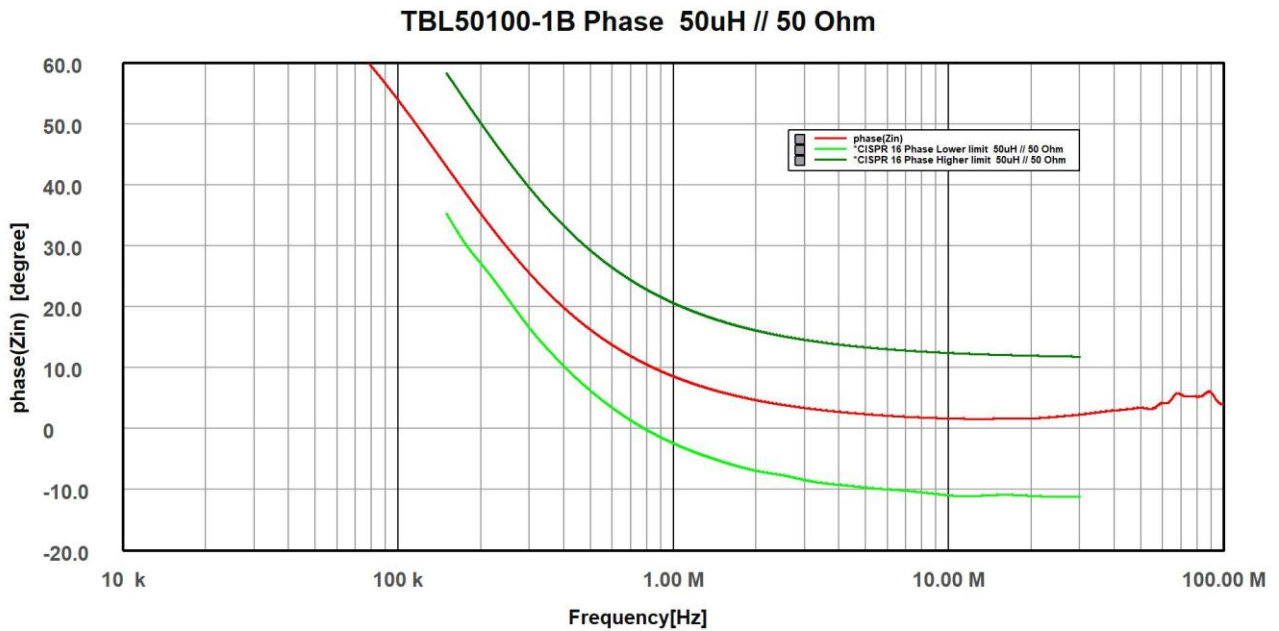
Picture 4: LISN phase, 50Ω // 50µH CISPR 16
