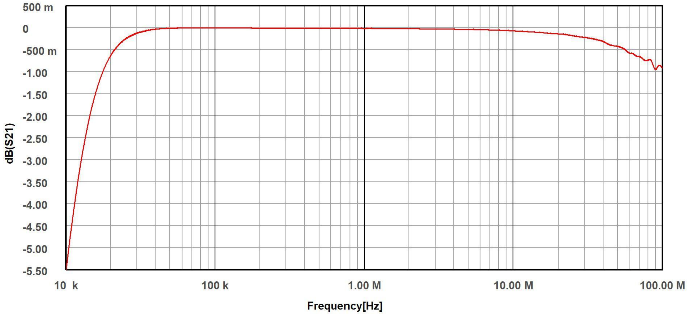
Picture 9: Voltage division ratio EUT terminals to RF connector, (50 \mu H + 5 \Omega ) // 50 \Omega , MIL-STD
