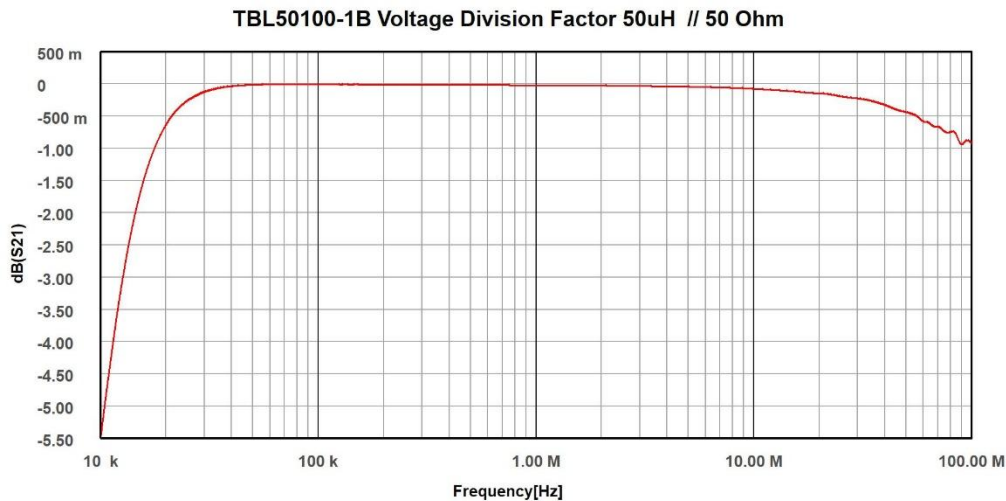
Picture 8: Voltage division ratio EUT terminals to RF connector, 50Ω // 50µH, CISPR 16
