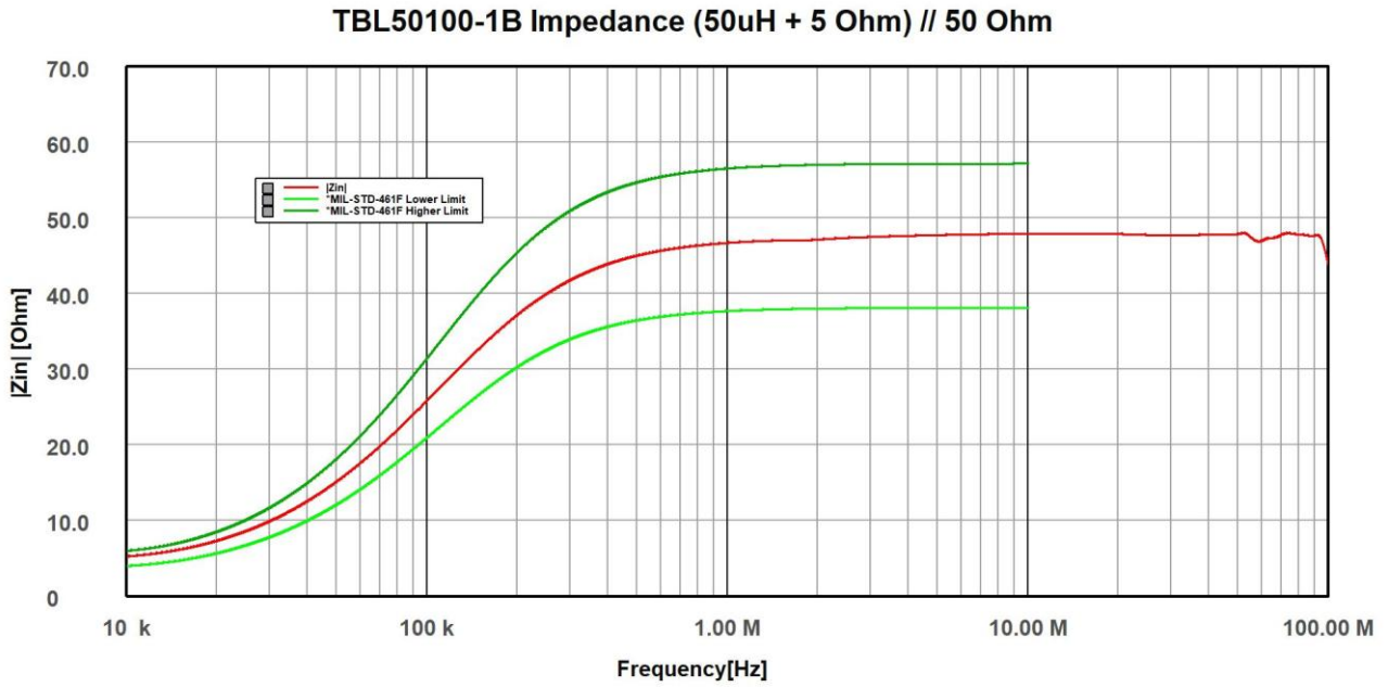
Picture 3: LISN impedance, (50µH + 5Ω) // 50 Ω MIL-STD
