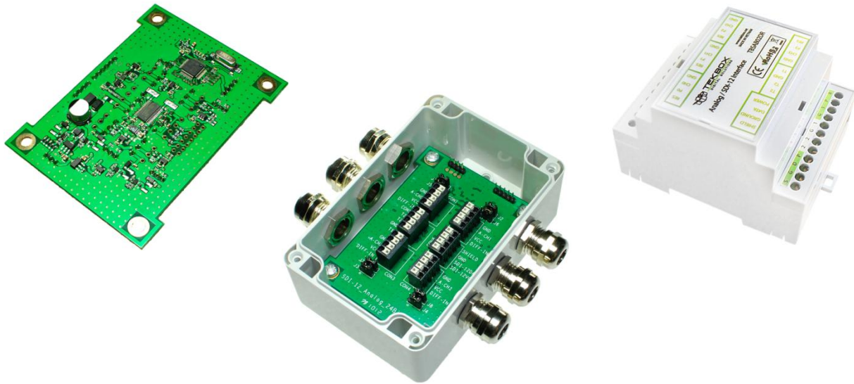
TBSAB02 4+1 Channel Analog to SDI-12 Interface
