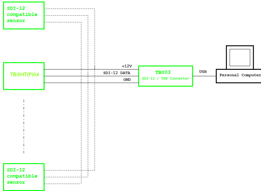
Figure 1 – TBSHT04/TBSHTP04 sensors connected to TBS03 SDI-12 to USB converter, setup for controlling / testing sensors and for PC based data recording
