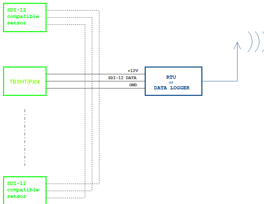
Figure 2 – TBSHT04/TBSHTP04 sensor(s) connected to Remote Telemetry Unit or Data Recorder
